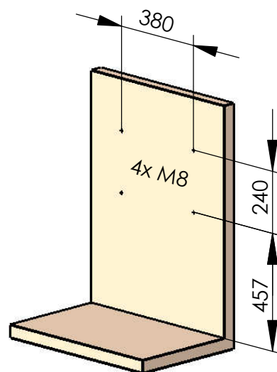
recommended hole pattern
